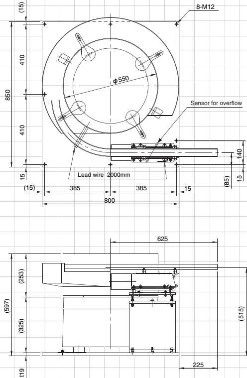
11 ER-55B+LFG-700
