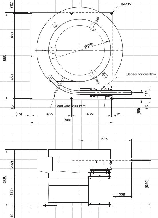
12 ER-65B+LFG-700
