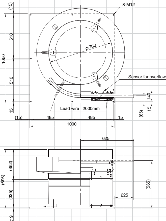
13 ER-75B+LFG-700
