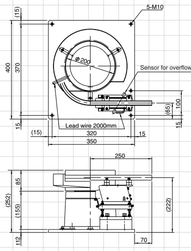
2 EA/DMS-20+LFB-300
