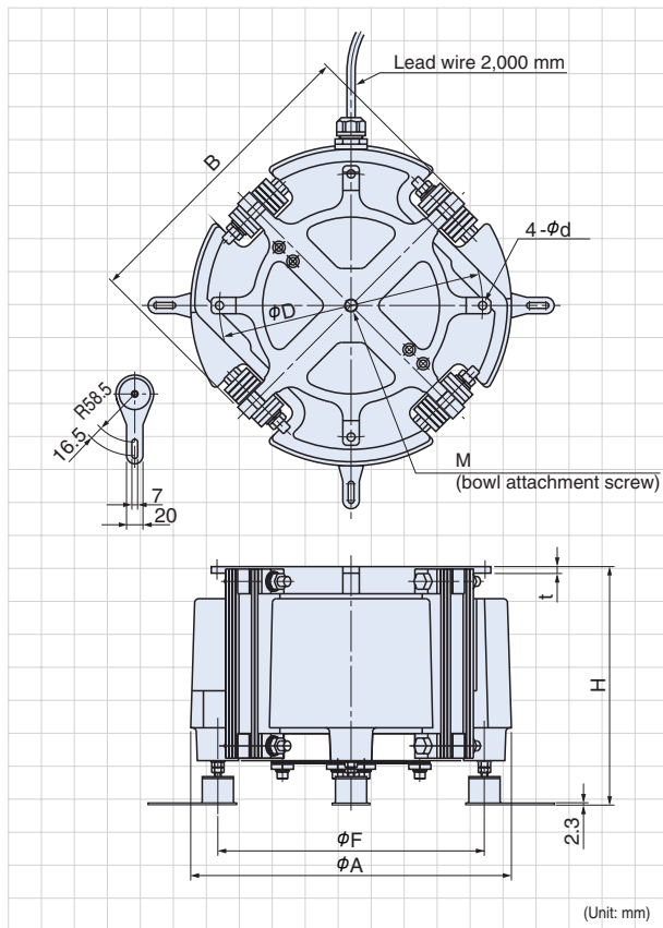
DM-30C~45C Dimensions
