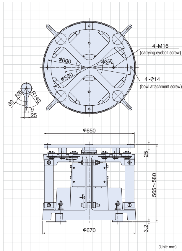
DM-65C Dimensions
